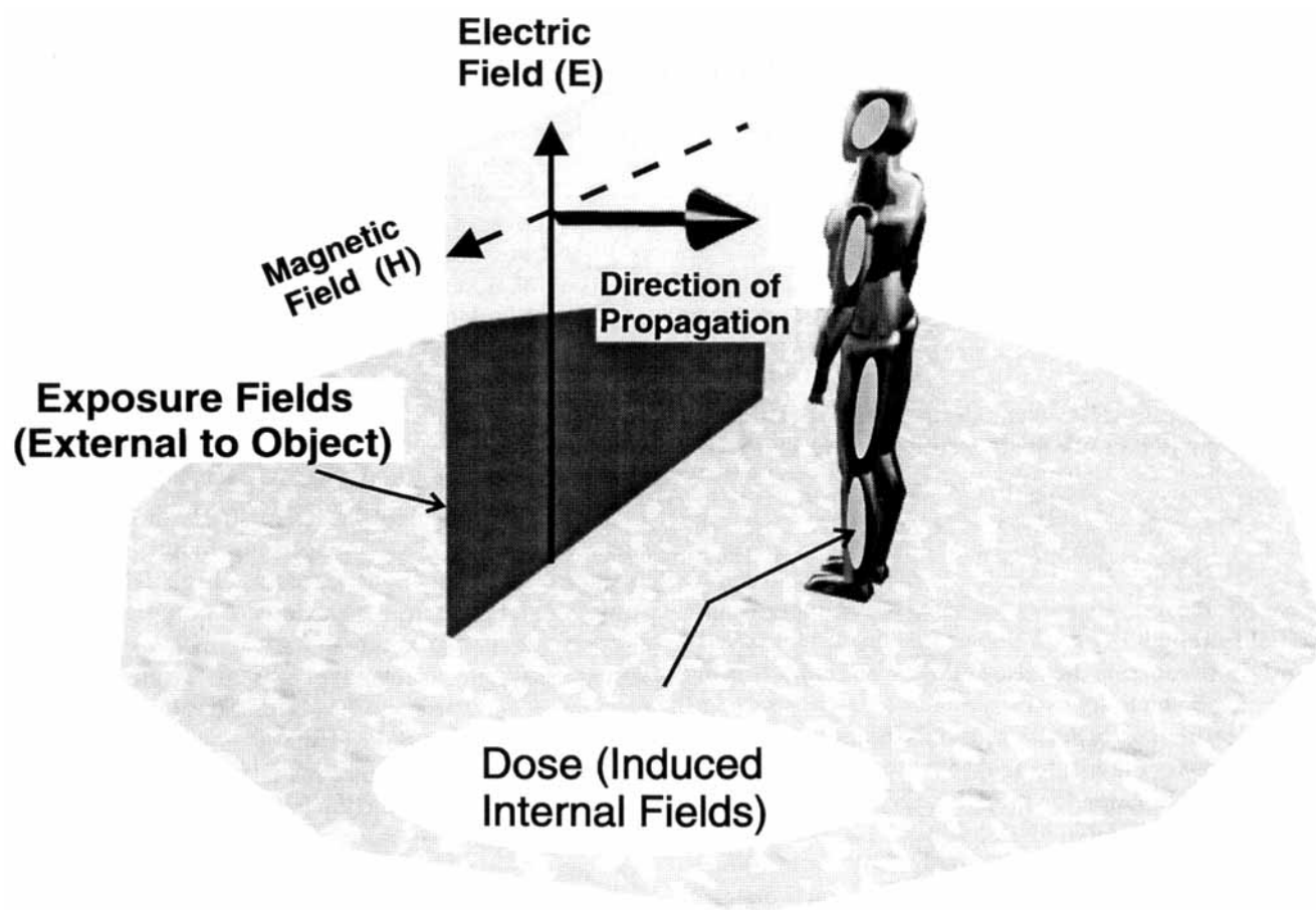
Fig. 1. Spatially uniform incident radio frequency (RF) fields and resulting nonuniform distribution of internal fields.
